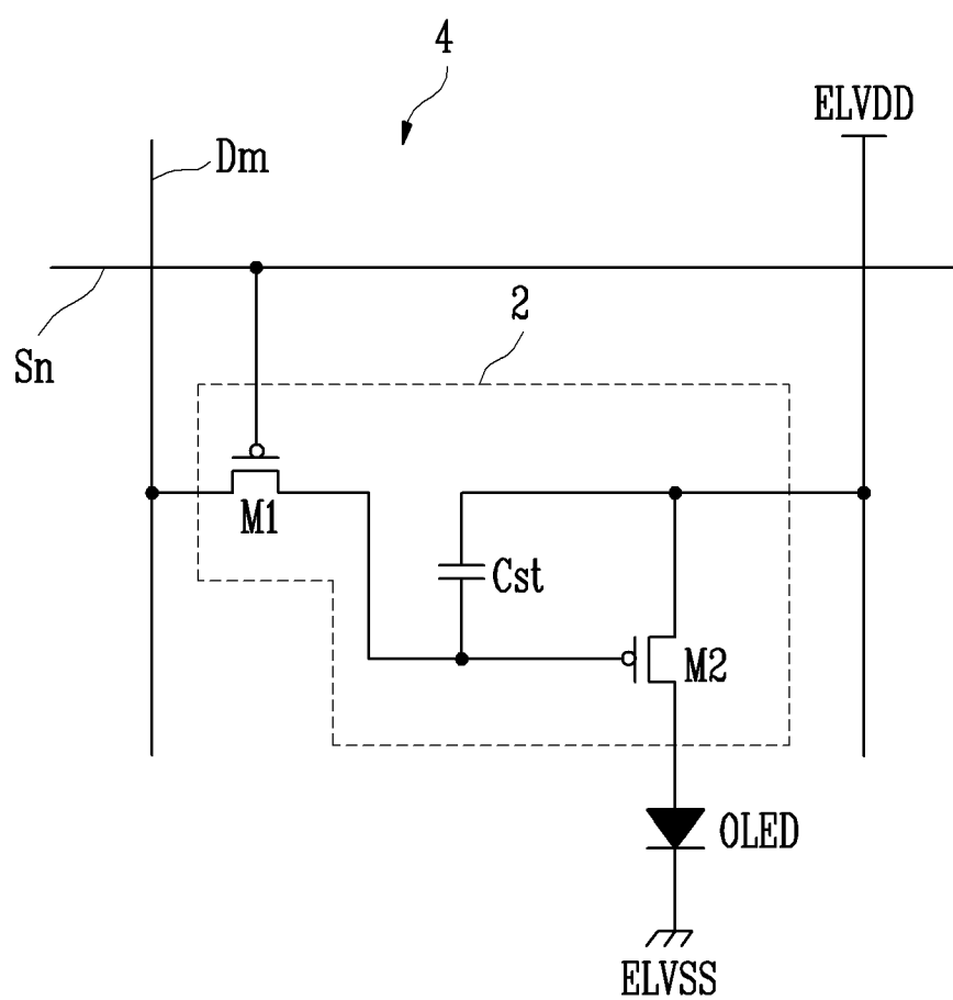
FIG. 1 (PRIOR ART)
