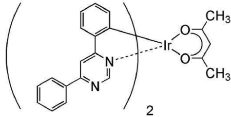
[Ir(dppm) 2 (acac)]
