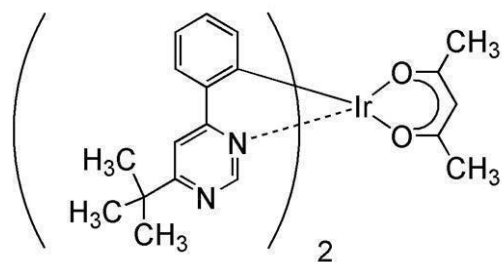
[Ir(tBuppm) 2 (acac)]
