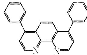
Bathophenanthroline
