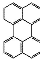
Perylene
