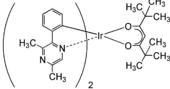
[Ir(mppr-Me) 2 (dpm)]
