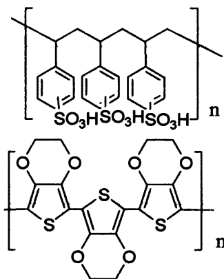
PEDOT-PSS
