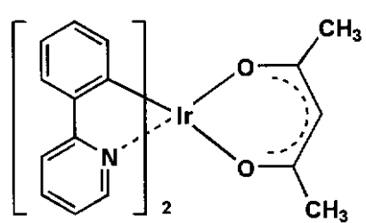
Ir-8
