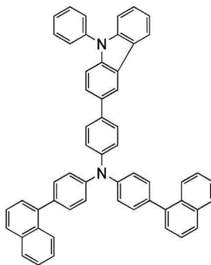
PCBNBB
