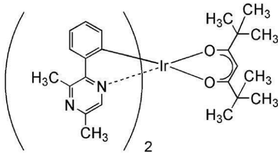
[Ir(mppr-Me) 2 (dpm)]
