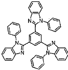
TPBi
