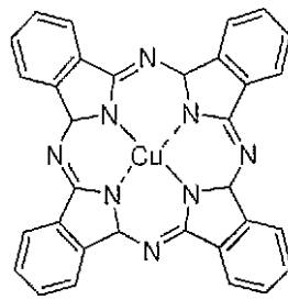
CuPc
