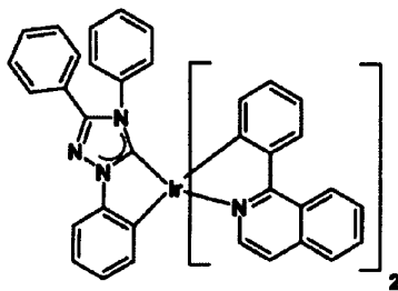
Complex A
