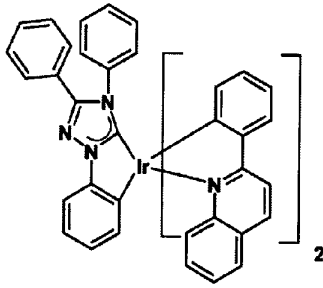
Complex B
