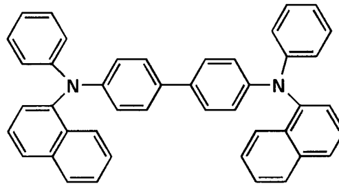
α-NPD
