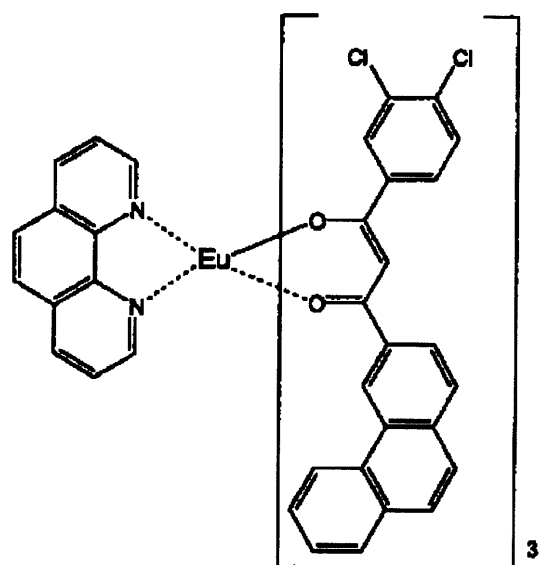
RE-15
