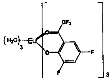
RF-6
