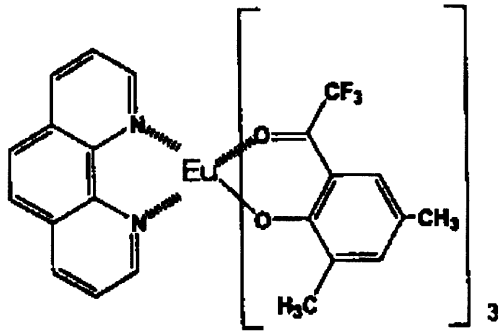
RF-1
