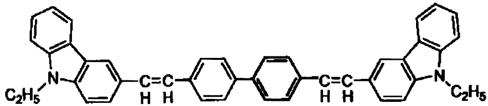
BCzVBi
