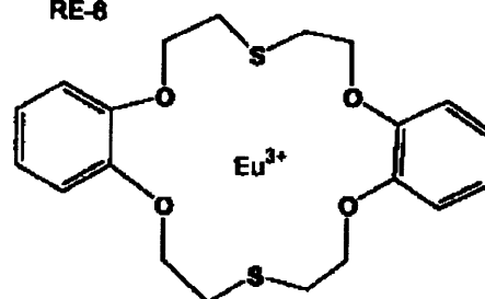
RE-8
