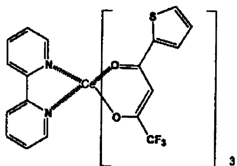
RE-12
