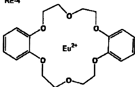
RE-4
