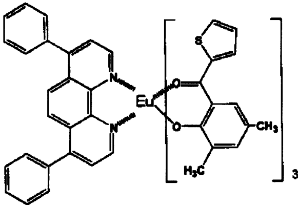
RF-2
