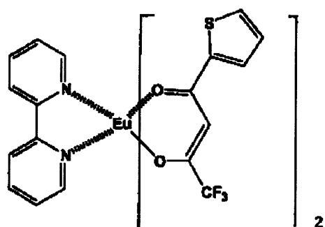
RE-10
