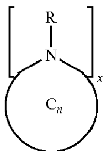
Azafulleroid
