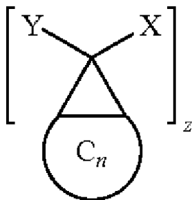
Bingel Derivative
