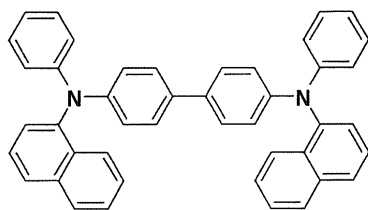
(102) α-NPD
