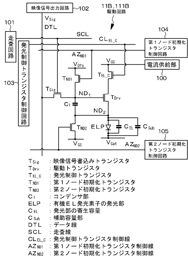
【図2】[5Tr/1C駆動回路]
