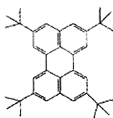
TBP
