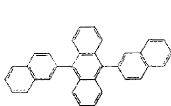
ADN
