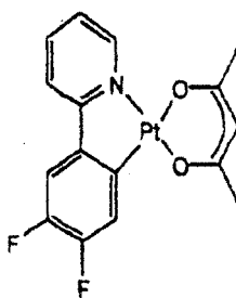
(4,5-F 2 ppy)Pt(acac)
