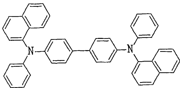
NPB
