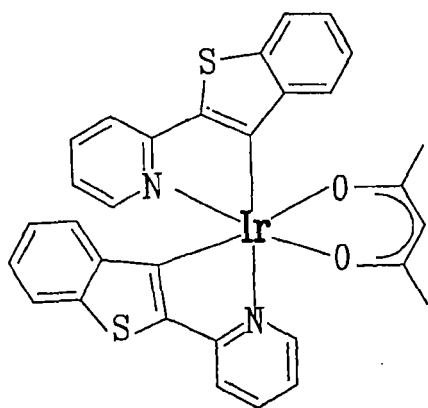
(btp) 2 Ir(acac)
