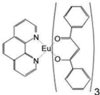
Eu(DBM) 3 (Phen)
