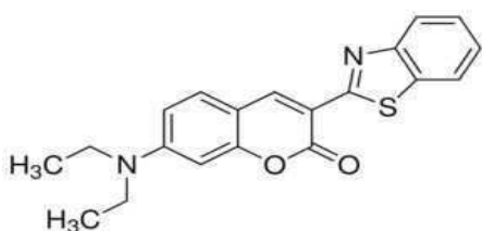
[0066] [0067] coumarin 6
