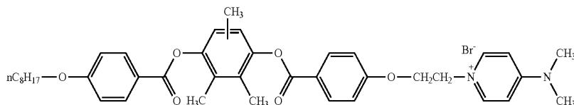
Pyridinium salt
