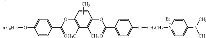
Pyridinium salt
