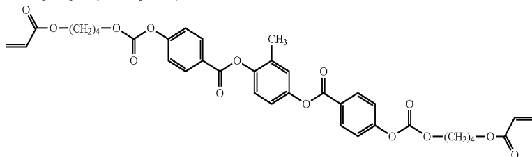
Fluorinated polymer
