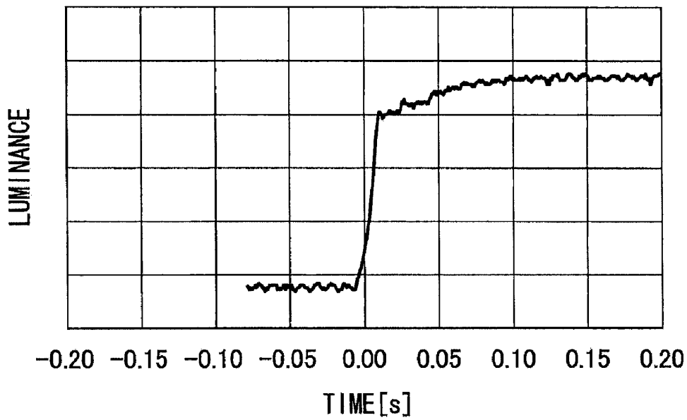
RESPONSE WAVEFORM 0→64
