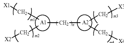
[Chemical Formula 7]
