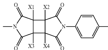
[Chemical Formula 5]
