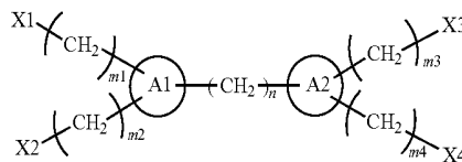
[Chemical Formula 7]
