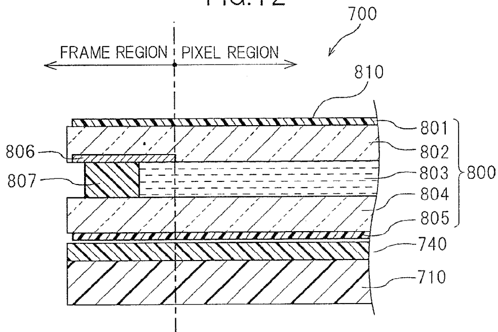
FIG. 12 (Prior Art)
