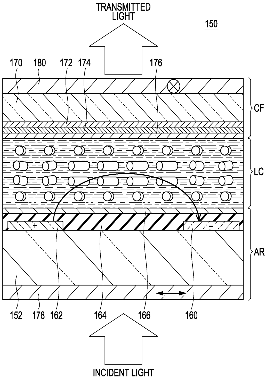
FIG. 23 PRIOR ART
