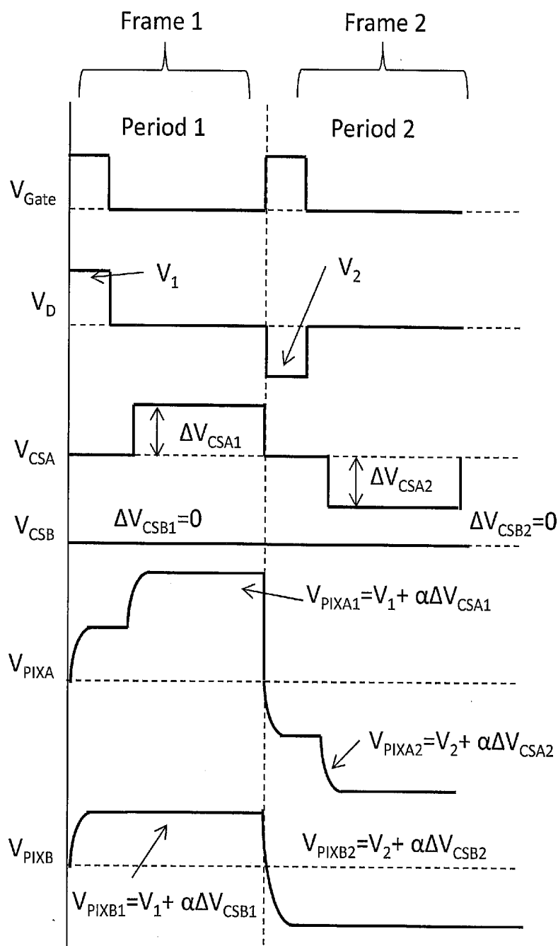
Figure 3 Conventional Art
