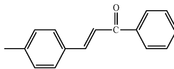
[Chem. 4]
