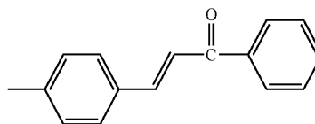
[Chem. 4]
