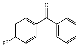
[Chem. 10]
