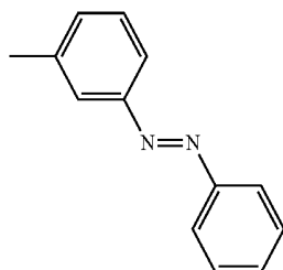
[Chem. 2]
