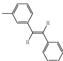
[Chem. 2]
