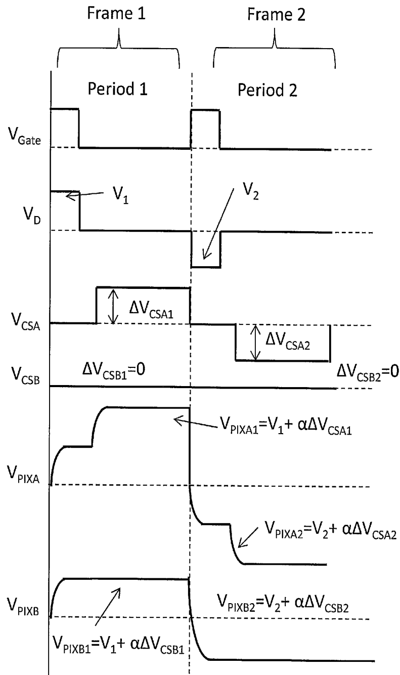
Figure 3 Conventional Art
