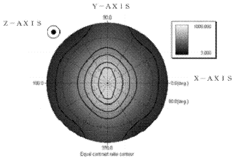
EQUAL CONTRAST CURVES FOR CONTRASTS OF 300, 200, 100, 50, AND 10 FROM THE INSIDE
