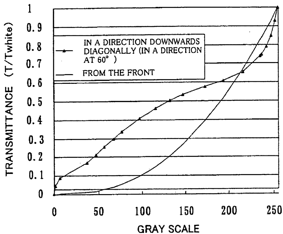
FIG. 2 (PRIOR ART)
