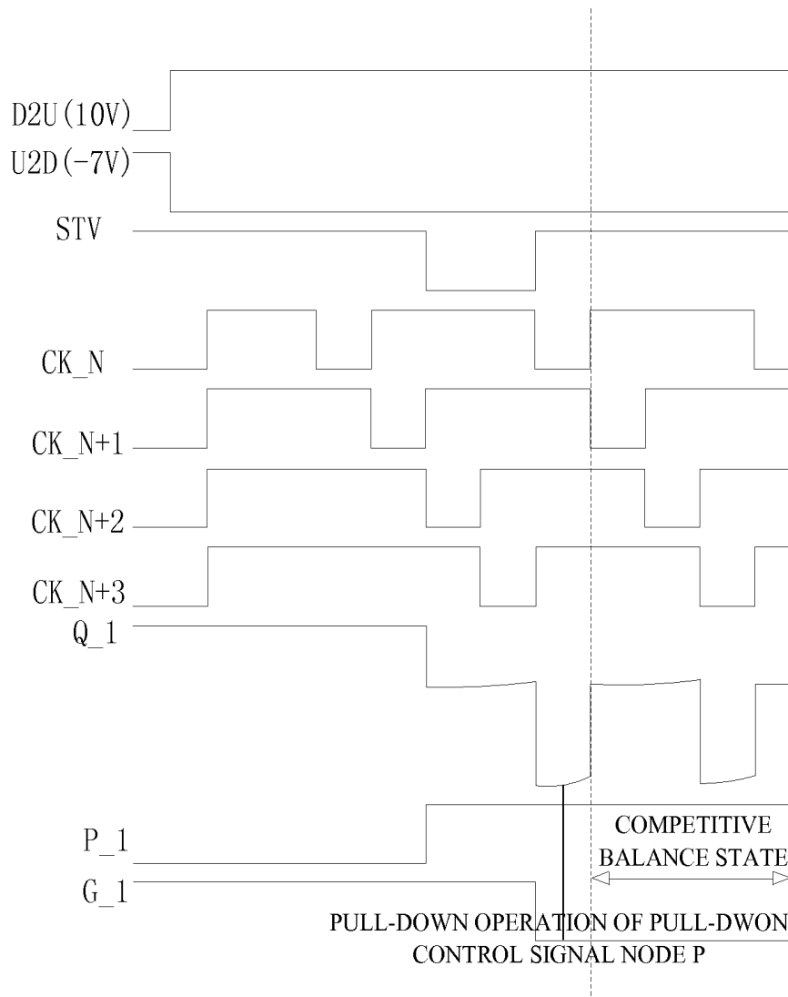
FIG. 2 (PRIOR ART)
