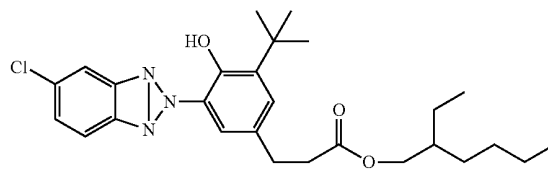
Structure of UV Absorbent A
