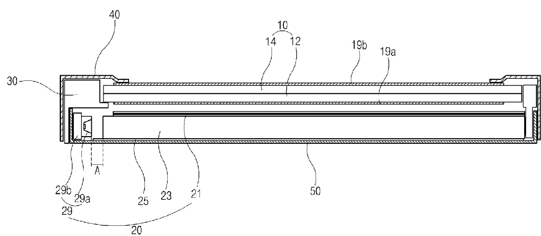
FIG. 1 Related Art
