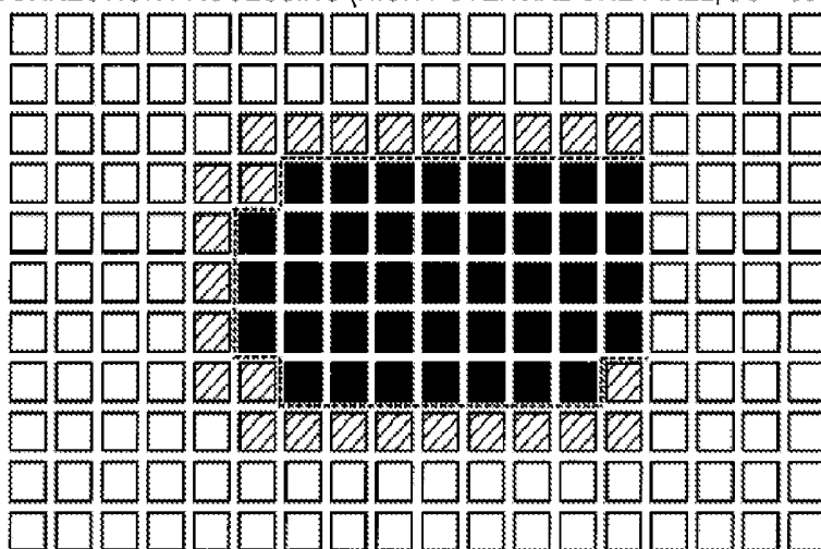
FIG. 16C CORRECTION PROCESSING (HIGH POTENTIAL ONE PIXEL, \theta_b = 225^\circ )
