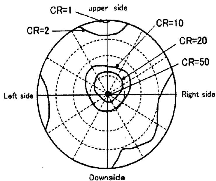
FIG. 2A(PRIOR ART)
