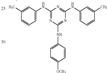
Compound 1
