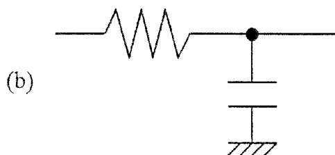
FIRST APPROXIMATION CIRCUIT OF CS BUSLINE LOAD IMPEDANCE: OR LOW PASS FILTER
