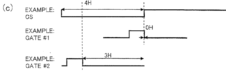
MINIMUM CYCLE (8H) OF Type II
