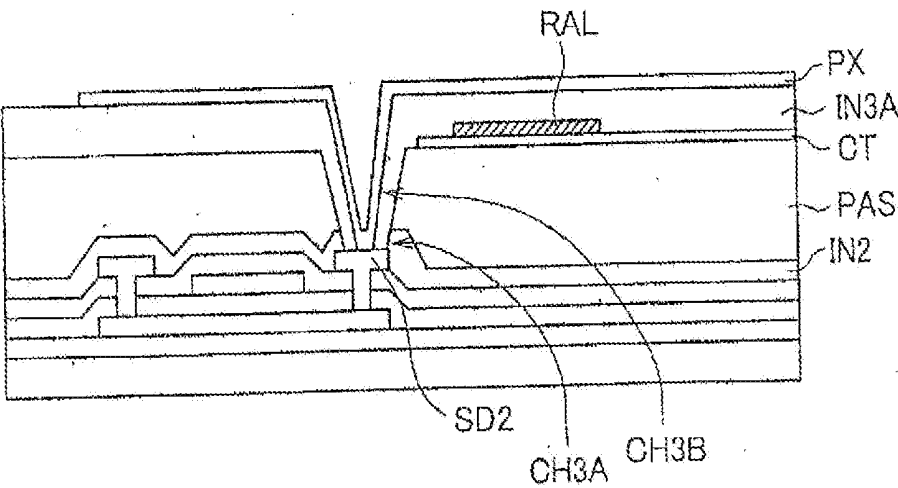
FIG. 7 RELATED ART
