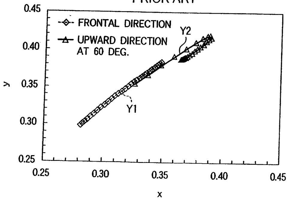
FIG.19 PRIOR ART
