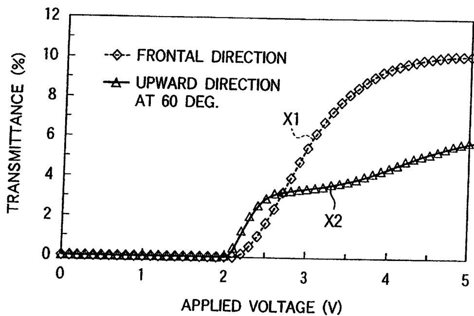
FIG.18 PRIOR ART
