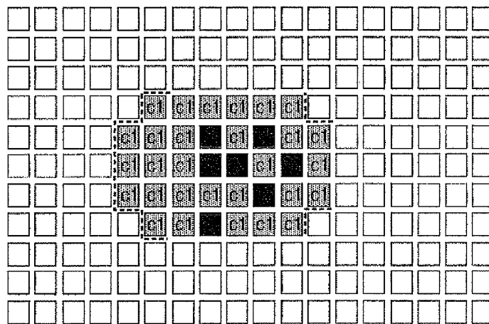
FIG. 16C CORRECTION PROCESS (THREE PIXELS ON LOW POTENTIAL SIDE; \theta_b=225^\circ )
