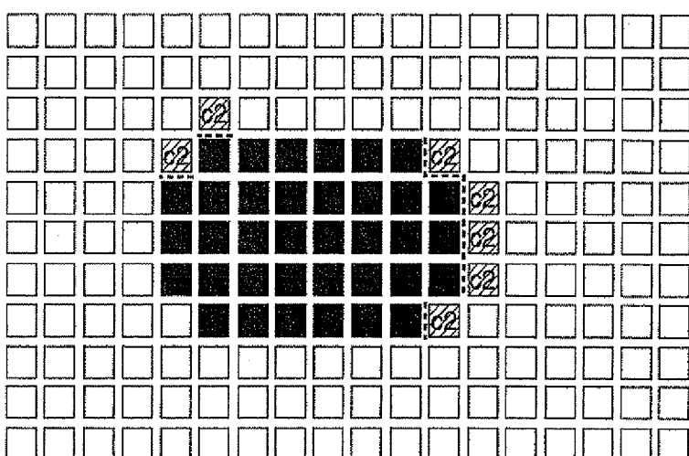
FIG. 17C CORRECTION PROCESS (ONE PIXEL ON HIGH POTENTIAL SIDE; \theta b=225^\circ )
