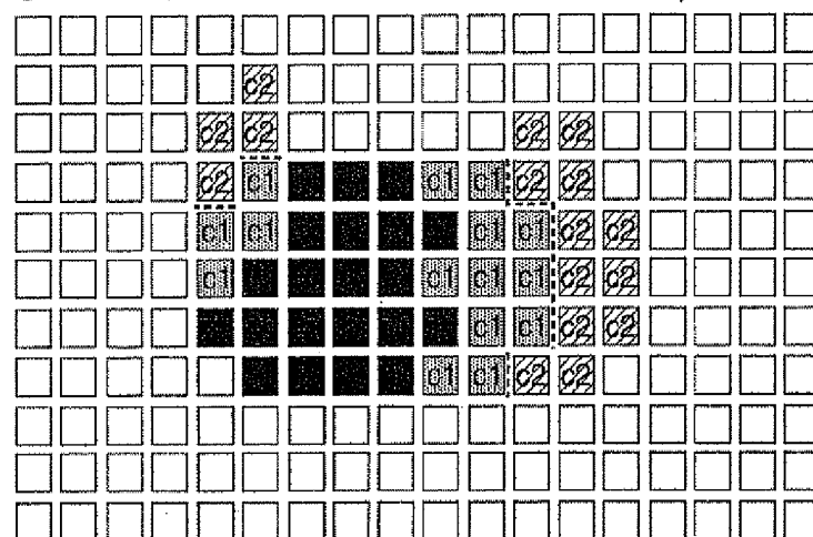
FIG. 21C CORRECTION PROCESS (TWO PIXELS ON LOW POTENTIAL SIDE +TWO PIXELS ON HIGH POTENTIAL SIDE; \theta_b=225^\circ )
