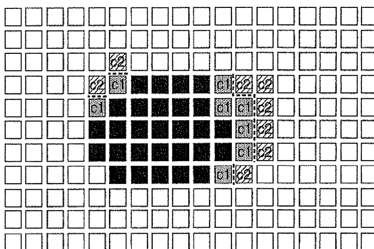
FIG. 20C CORRECTION PROCESS (ONE PIXEL ON LOW POTENTIAL SIDE +ONE PIXEL ON HIGH POTENTIAL SIDE; \theta_b=225^\circ )
