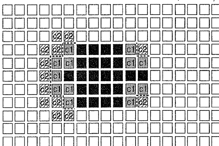
FIG. 20B CORRECTION PROCESS (ONE PIXEL ON LOW POTENTIAL SIDE +ONE PIXEL ON HIGH POTENTIAL SIDE; \theta_b=90^\circ )
