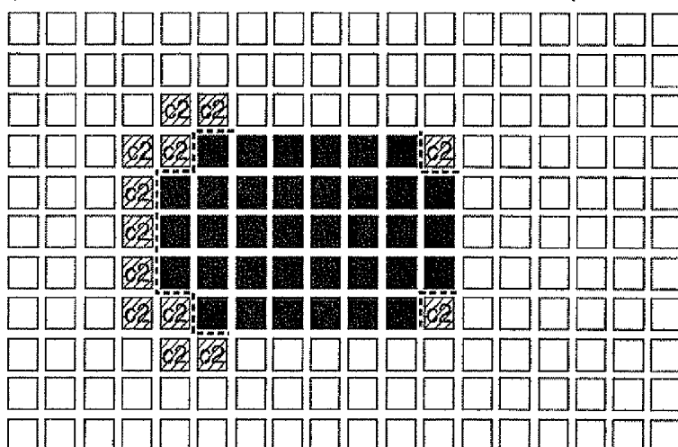
FIG. 17B CORRECTION PROCESS (ONE PIXEL ON HIGH POTENTIAL SIDE; \theta b=90^\circ )
