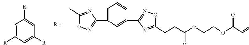
Compound 102
