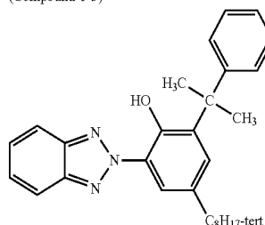
(Compound 1-3)
