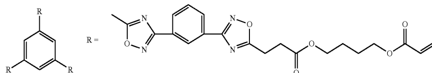
Compound 101
