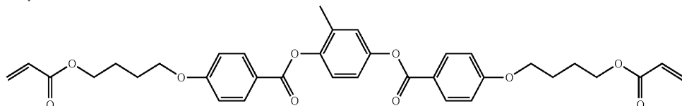
Rod-like compound 18-1
