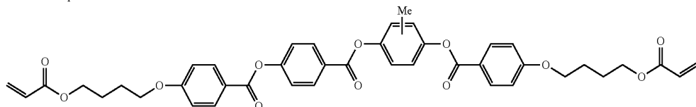
Rod-like compound 18-2
