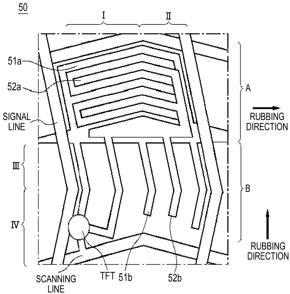
FIG.10 PRIOR ART
