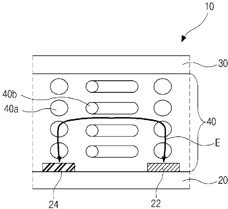
(related art) FIG. 1A
