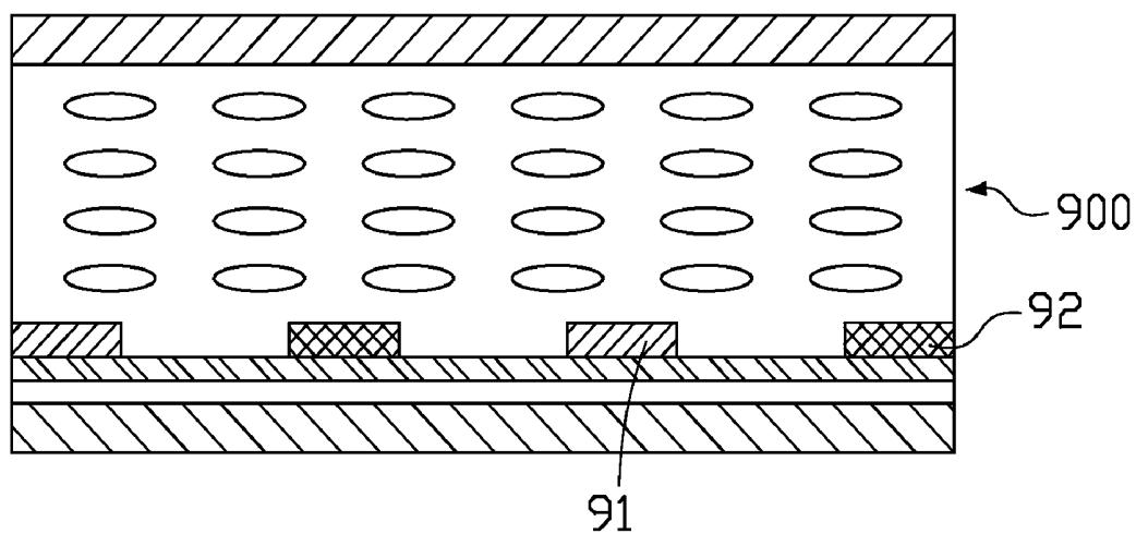
FIG. 2 (PRIOR ART)
