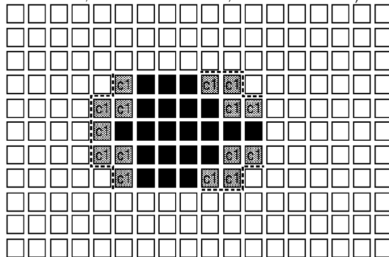
FIG. 14B CORRECTION PROCESS (LOW ELECTRIC POTENTIAL, ONE TARGET PIXEL, \theta_b = 90 DEGREES)
