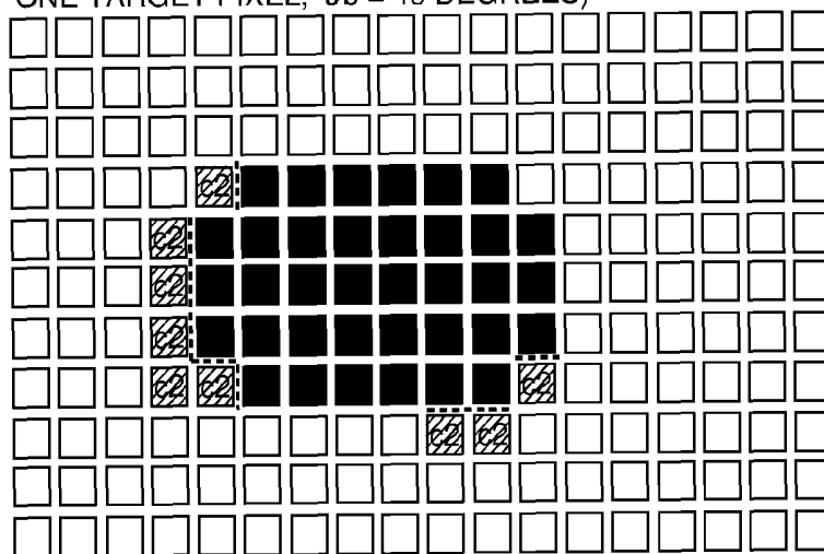
FIG. 21B CORRECTION PROCESS (HIGH ELECTRIC POTENTIAL, ONE TARGET PIXEL, \theta_b = 90 DEGREES)
