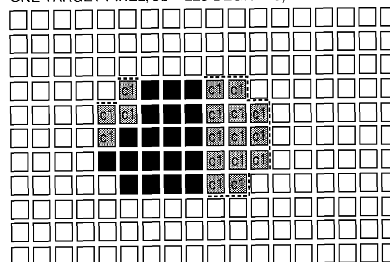
FIG. 19C CORRECTION PROCESS (LOW ELECTRIC POTENTIAL, ONE TARGET PIXEL, \theta_b = 225 DEGREES)
