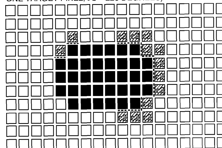
FIG. 21C CORRECTION PROCESS (HIGH ELECTRIC POTENTIAL, ONE TARGET PIXEL, \theta_b = 225 DEGREES)
