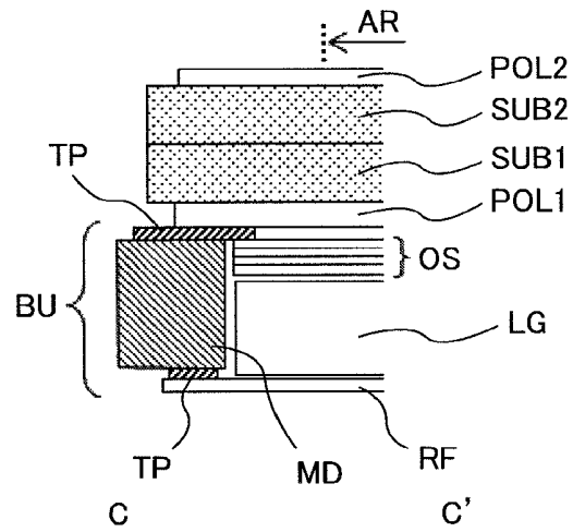
FIG. 7 PRIOR ART
