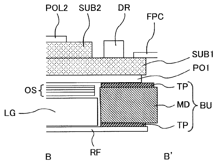
FIG. 6 PRIOR ART
