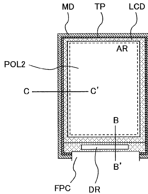
FIG. 5 PRIOR ART
