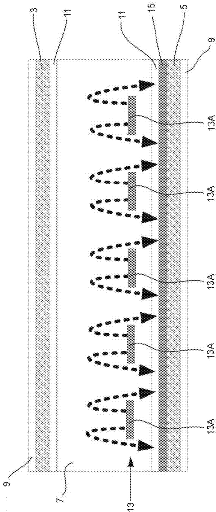
FIG.1 PRIOR ART
